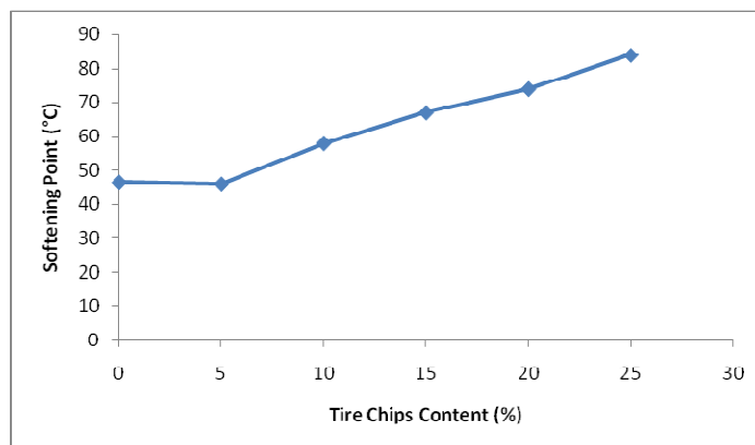
Fig.3.3: Variation of Softening Point with Tire Chips Content
