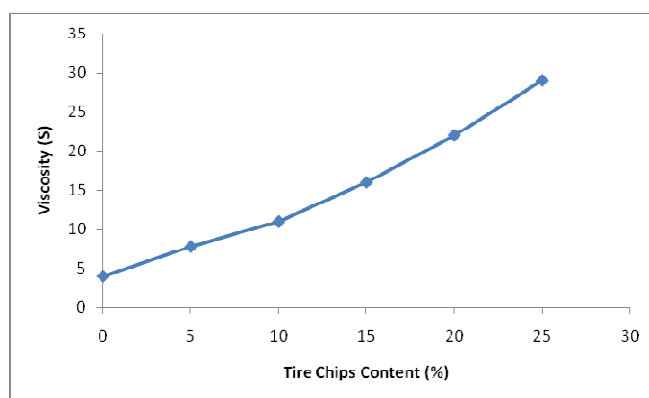
Fig.3.4: Variation of Viscosity with Tire Chips Content
