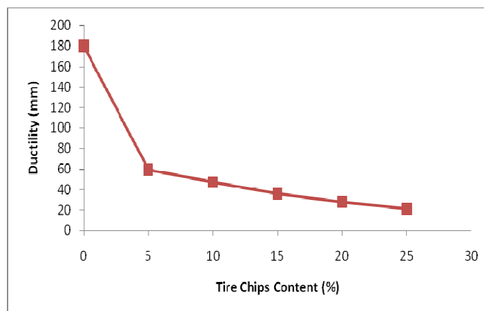
Fig. 3.2: Variation of Ductility with Tire Chips
