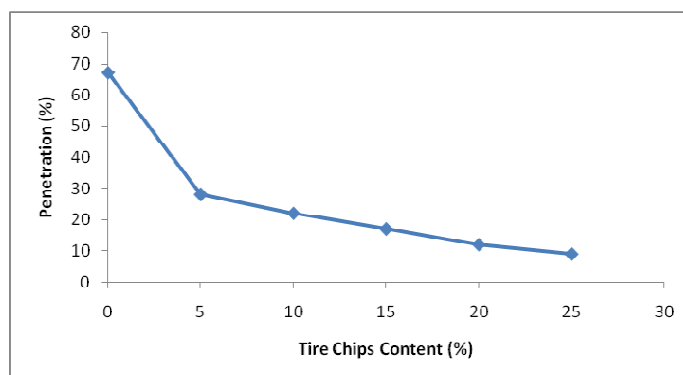
Fig.3.1: Variation of penetration with tire chips content
